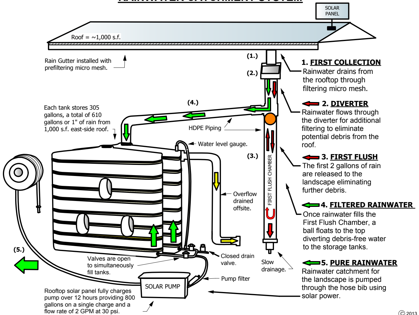
610 Gallon Storage
